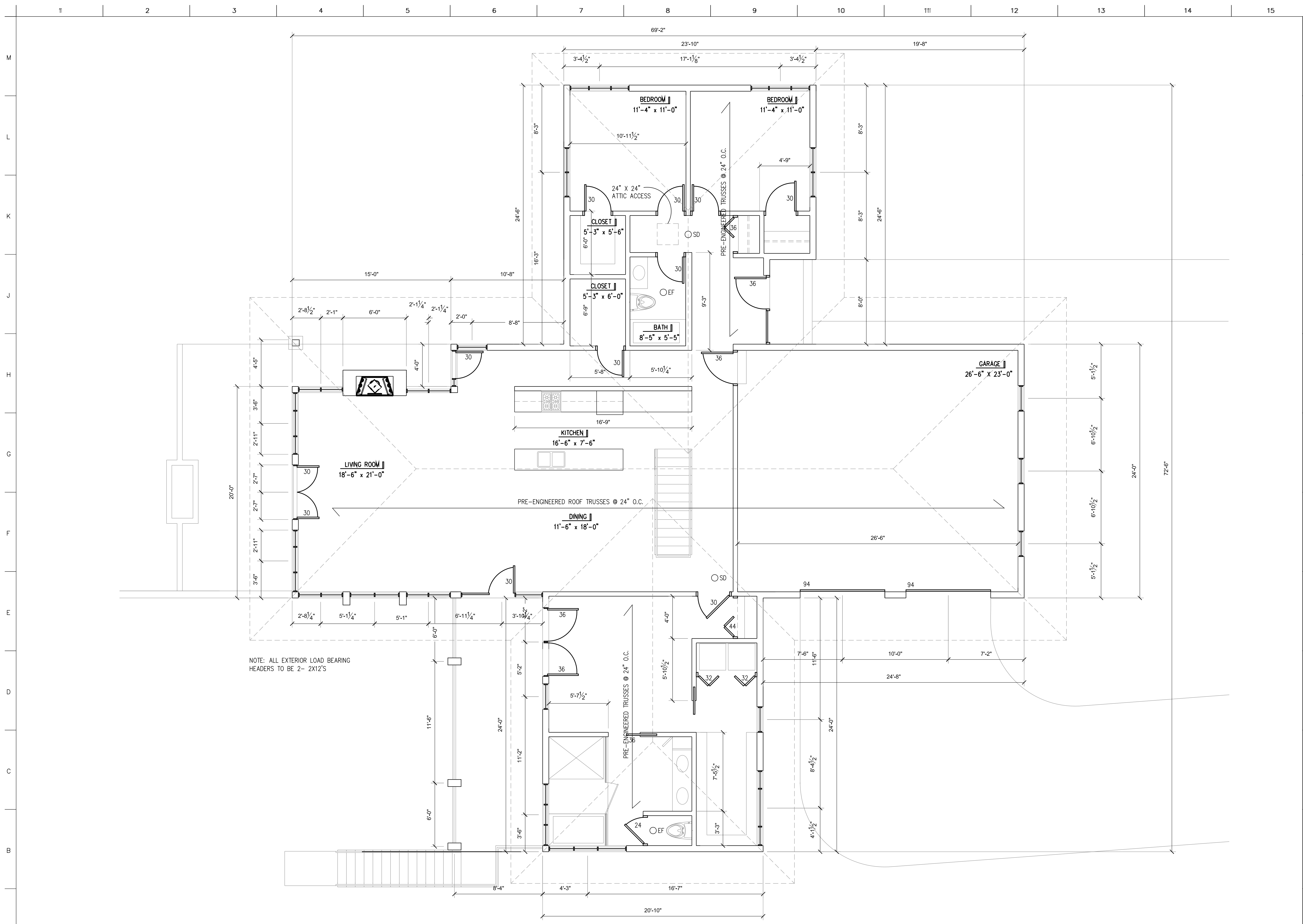
A1 FIRST LEVEL FLOOR PLAN SCALE: 1/4" = 1'-0"
