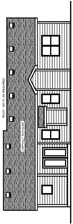
REAR ELEVATION
